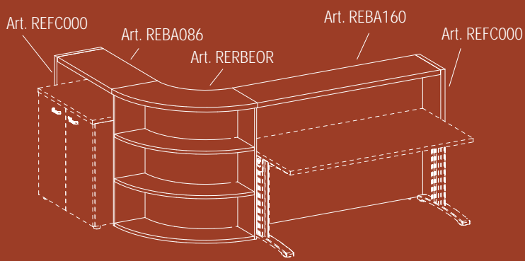
RECEPTION CON ANGOLO INTERNO PER MOBILI RECEPTION WITH INTERNAL ANGLE FOR WALL UNITS
